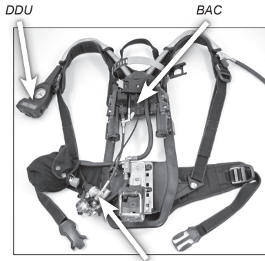
Manifold assembly
